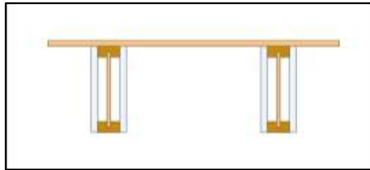
Figure 2a: end view of the installation of 12.5 mm (1/2 in.) regular gypsum board flange-to-flange of I-joist
