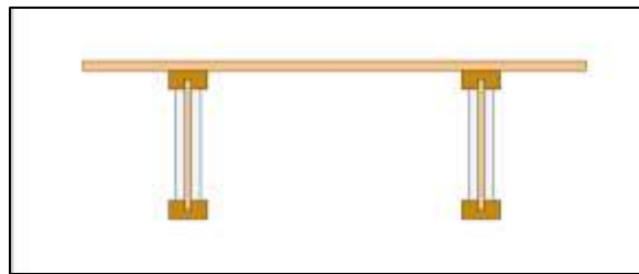
Figure 1a: end view of the installation of 12.5 mm (1/2 in.) regular gypsum board to protect web of I-joist
