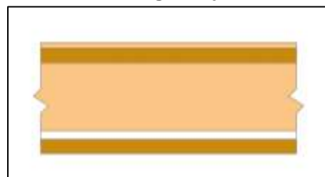
Figure 3b: side view for wood I-joist at 600 mm spacing, placing 15.8 mm (5/8 in.) regular gypsum board on top of bottom flange of I-joist
