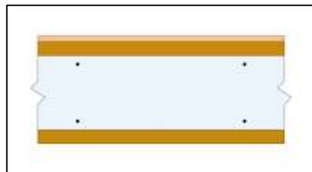
Figure 1b: side view of the installation of 12.5 mm (1/2 in.) regular gypsum board to protect web of I-joist
